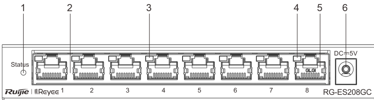
Figure 1-23 Front Panel of RG-ES208GC
