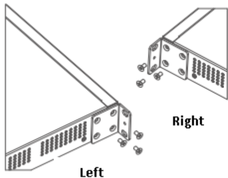
Figure 3-3 Attaching the Mounting Bracket to RG-ES224GC/RG-ES216GC
