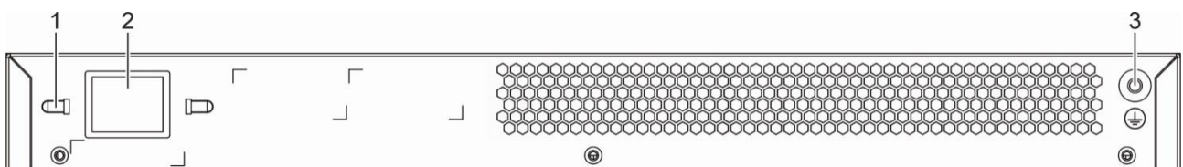
Figure 1-15 Back Panel of RG-ES224GC
