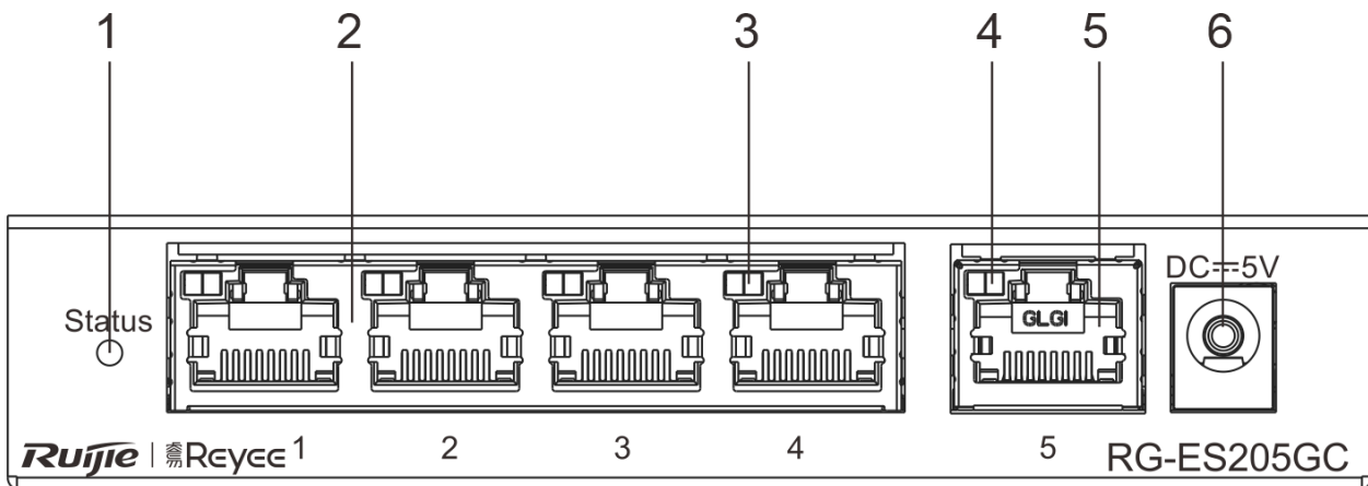
Figure 1-20 Front Panel of RG-ES205GC
