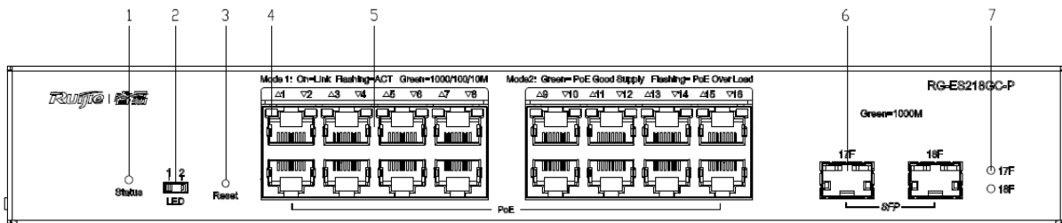
Figure 1-8 Front Panel of RG-ES218GC-P
