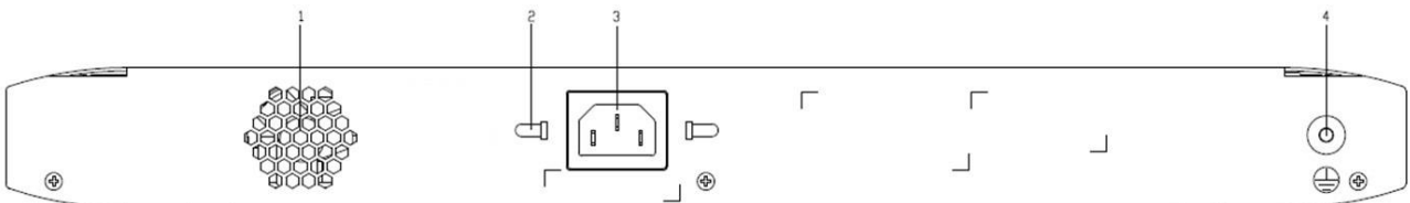
Figure 1-12 Back Panel of RG-ES226GC-P
