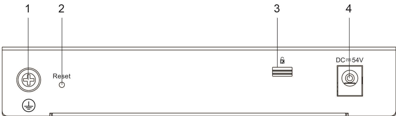
Figure 1-27 Back Panel of RG-ES206GC-P
