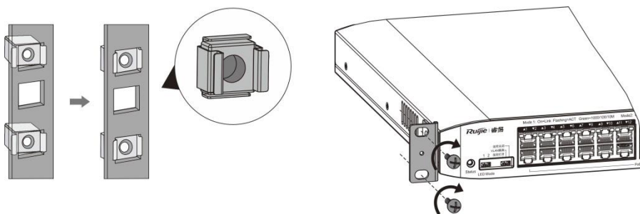
Figure 3-5 Attaching the Brackets to the Rack
