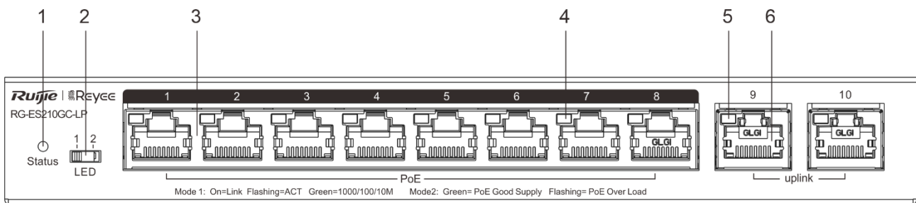
Figure 1-29 Front Panel of RG-ES210GC-LP
