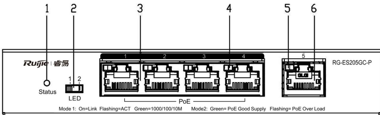
Figure 1-2 Front Panel of RG-ES205GC-P
