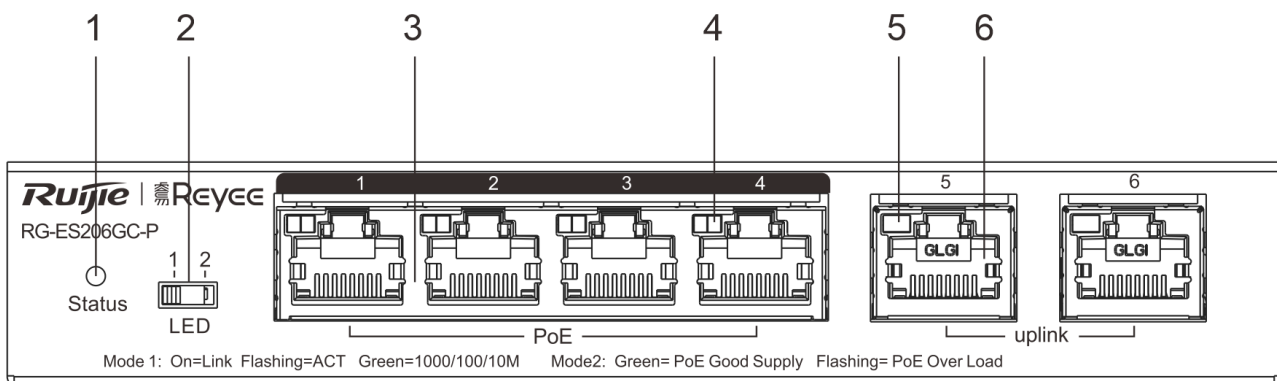
Figure 1-26 Front Panel of RG-ES206GC-P
