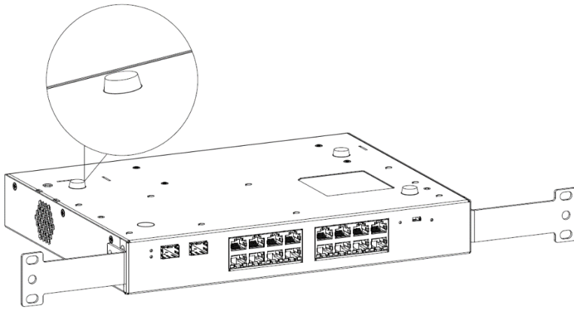
Figure 3-8 Attaching the Rubber Pads to the Recessed Areas
