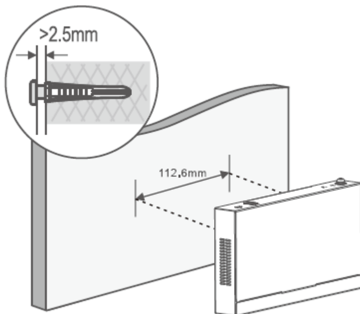
Figure 3-6 Mounting Switch on the Wall
