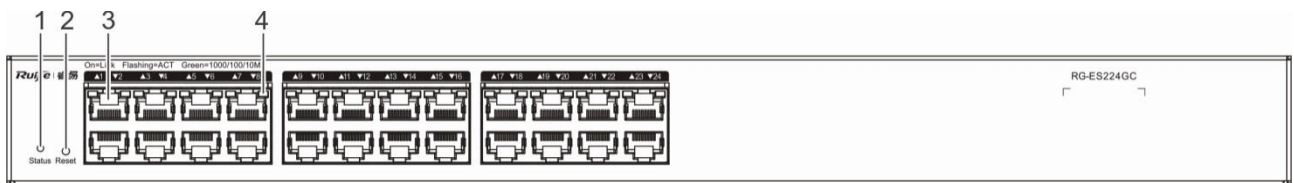
Figure 1-14 Front Panel of RG-ES224GC
